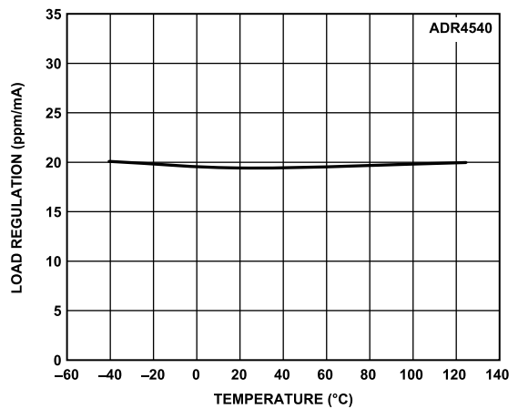
Figure 70. ADR4540 Load Regulation vs. Temperature (Sourcing)
