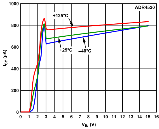
Figure 11. ADR4520 Supply Current ( I_{SY} ) vs. Supply Voltage
